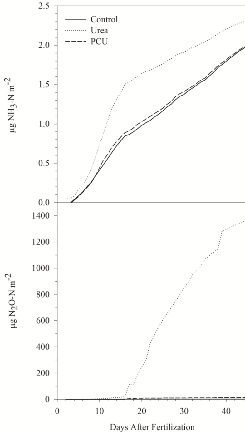
Figure 4. Total N Loss from N 2 O Emission and NH 3 Volatilization in 45 Day Study. The total N loss from urea treatments was consistently significantly higher than the PCU treatments.
