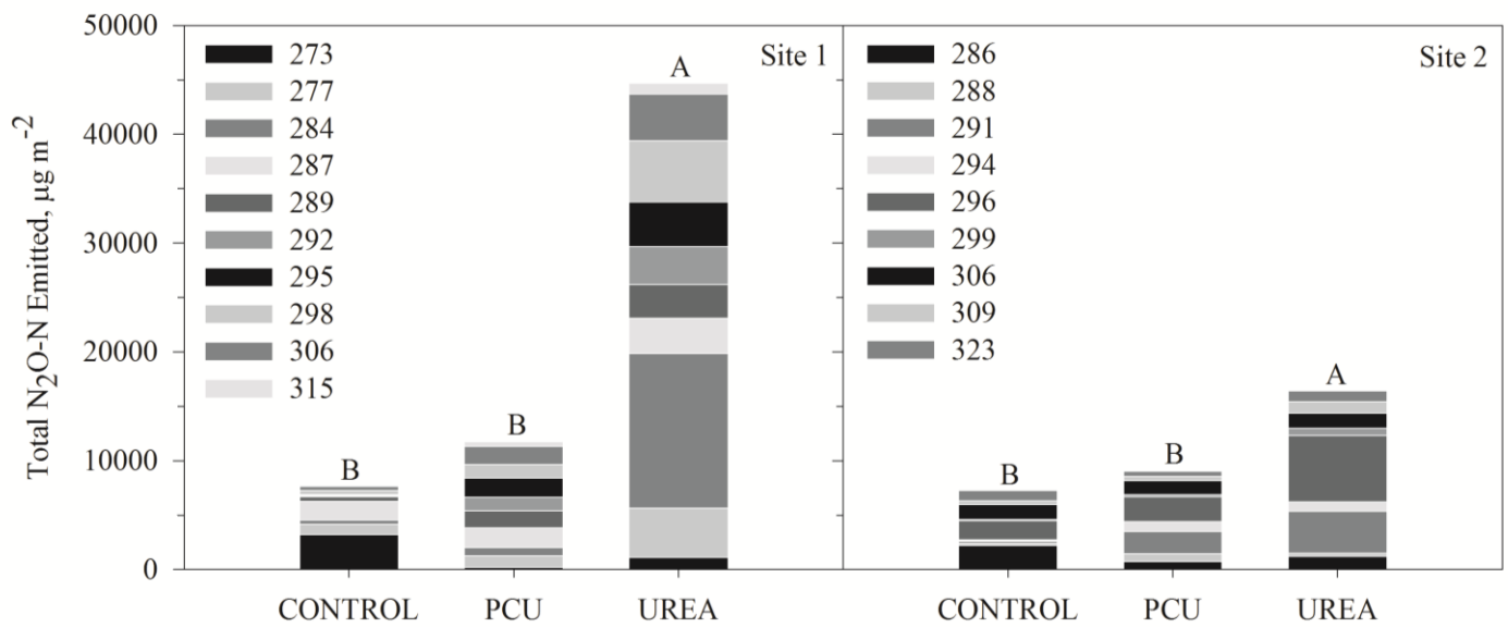
Figure 2. Cumulative N 2 O flux for the field sites from equivalent rates of (200 kg ha -1 N) urea and polymer coated urea (PCU) over a period of 45 days after application. Those treatments not sharing the same letter indicate significant differences ( P = 0.05 ).
