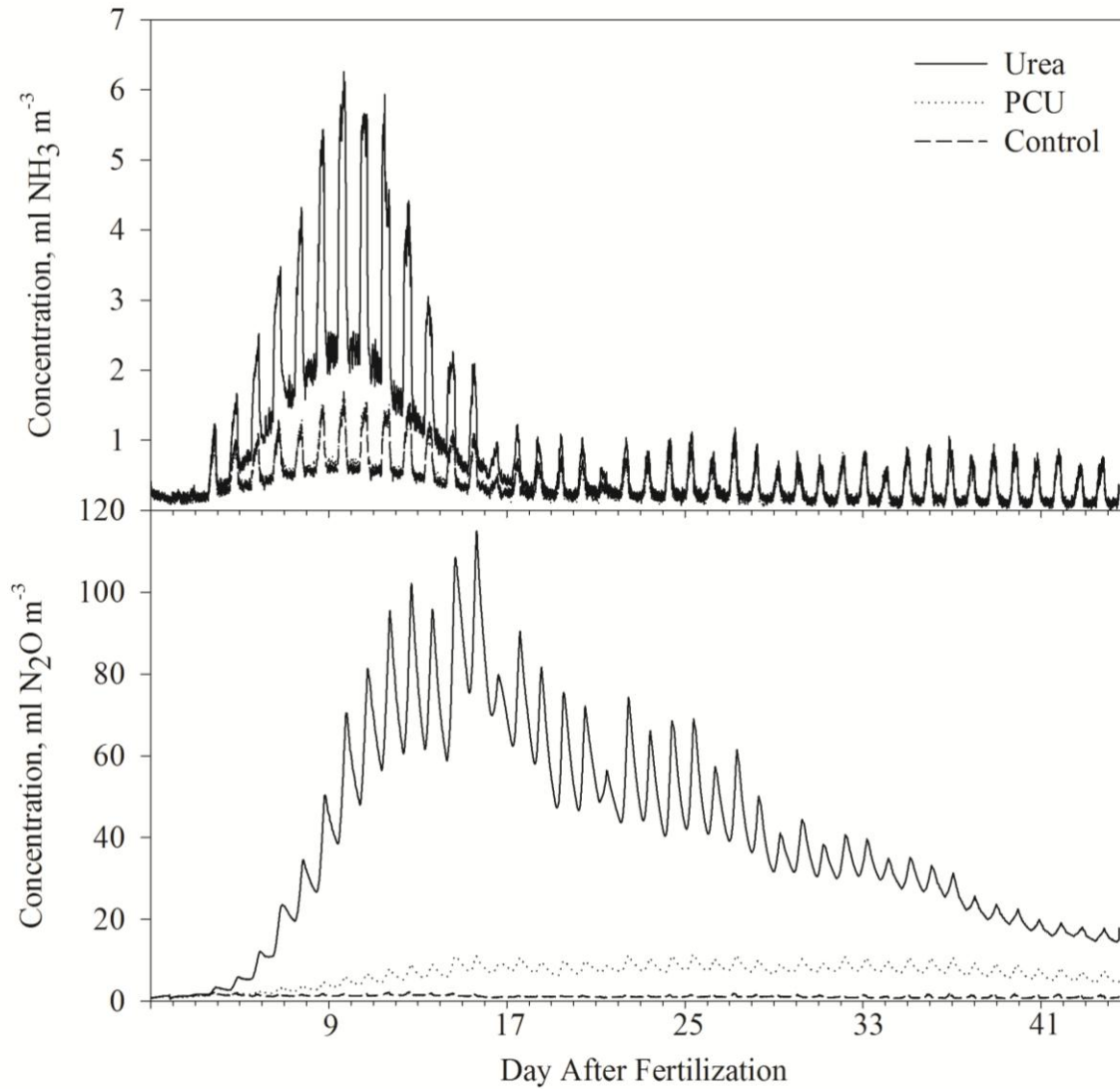
Figure 2. Concentration of N_2O and NH_3 in chamber headspace for 45 D Study. Samples were collected and analyzed every 11 min. to give this high-resolution view of the changes in concentration over time. These values were used to find the daily maximum concentration and the daily minimum which occurred prior to the maximum to estimate flux. Each day was analyzed individually and the statistics are reported in Table 2.
