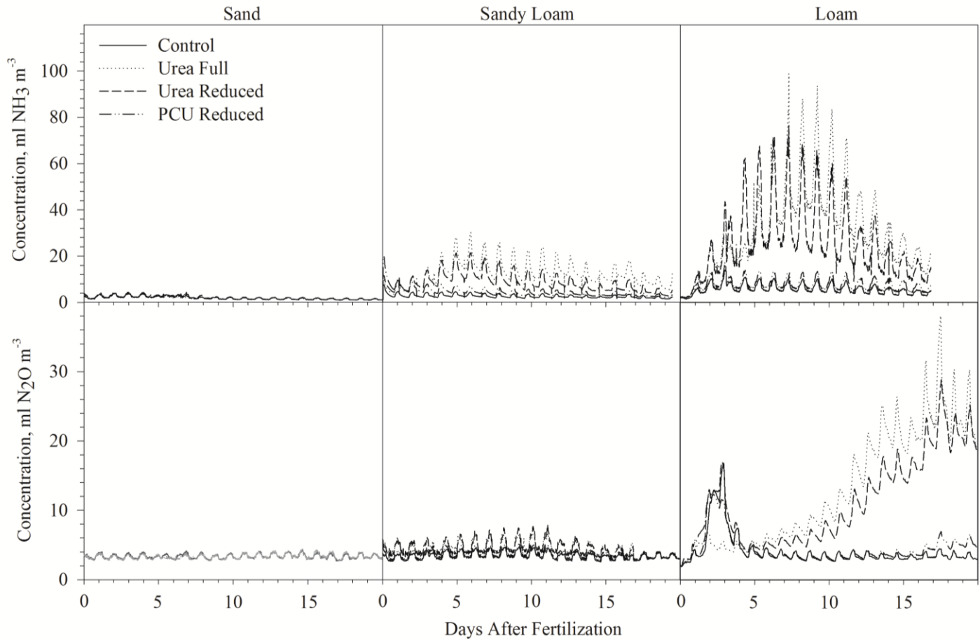
Figure 1. Concentration of N_2O and NH_3 in chamber headspace for 21 D Studies. Samples were collected and analyzed every 30 min. to give this high-resolution view of the changes in concentration over time. These values were used to find the daily maximum concentration and the daily minimum which occurred prior to the maximum to estimate flux. Each day was analyzed individually and the statistics are reported in Table 2.
