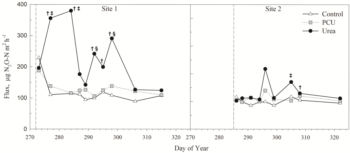
Figure 1. Daily N 2 O Flux for Sites 1 and 2. Significance indicated by † (urea greater than control), ‡ (urea greater than PCU), and § (PCU greater than control). Vertical dashed lines indicate fertilizer application.
